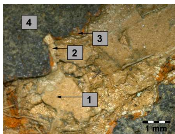
Figure 5 Optical micrograph detail of fragment V, with arrows and numbers marking the different layers: earthen render (1), white ground (2), red paint layer (3), and soot layer (4).
