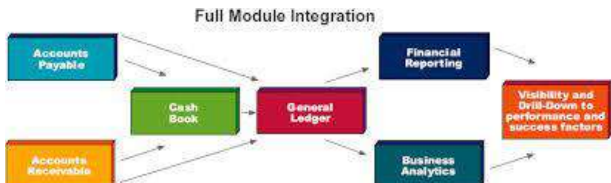
Figure 33: software modules
