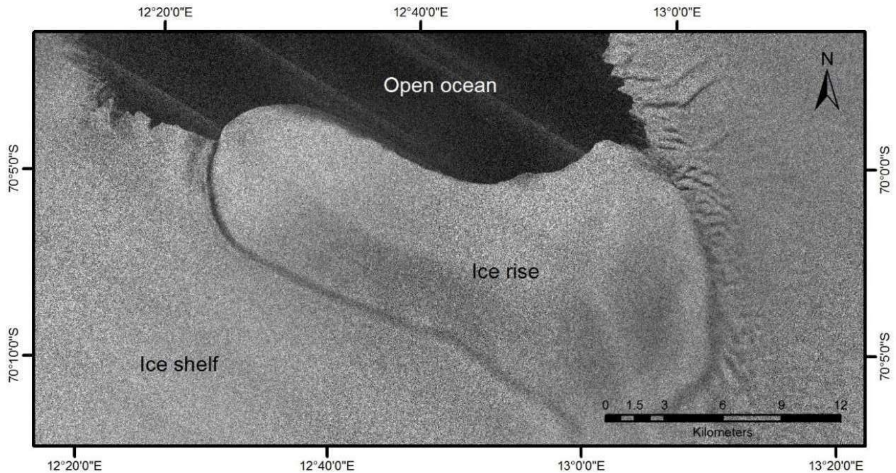
Figure 2.36: A satellite view covering ice rise near Lazarev Ice Shelf (RISAT-1; MRS; RH; 20 February 2016).
