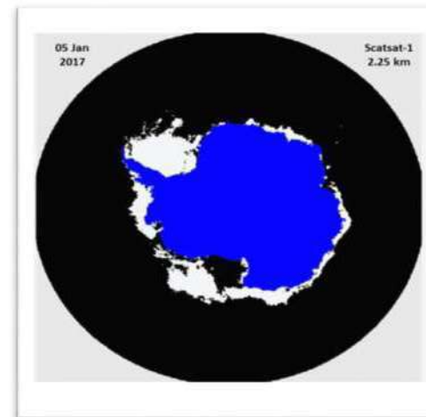
Figure 3.4: SCATSAT-1 derived sea ice extent (Source: http://vedas.sac.gov.in ).
