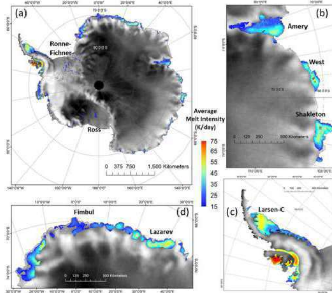
Figure 3.14: Average melt observed using SCATSAT-1 BT data over (a) Antarctic ice shelves for the study period (b) region covering Amery Ice Shelf, (c) region covering Antarctic Peninsula and (d) region covering Fimbul Ice Shelf.
